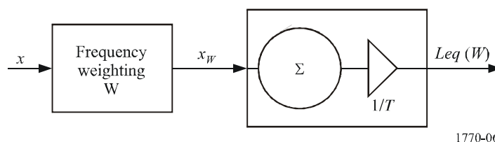
Block diagram of the simple energy-based loudness measures
